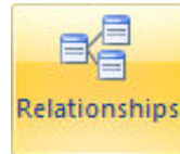
Fig. 2 Relationships button.
