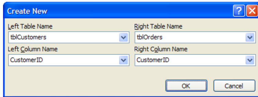
Fig. 6 Specifying related fields using the Create New dialog box
