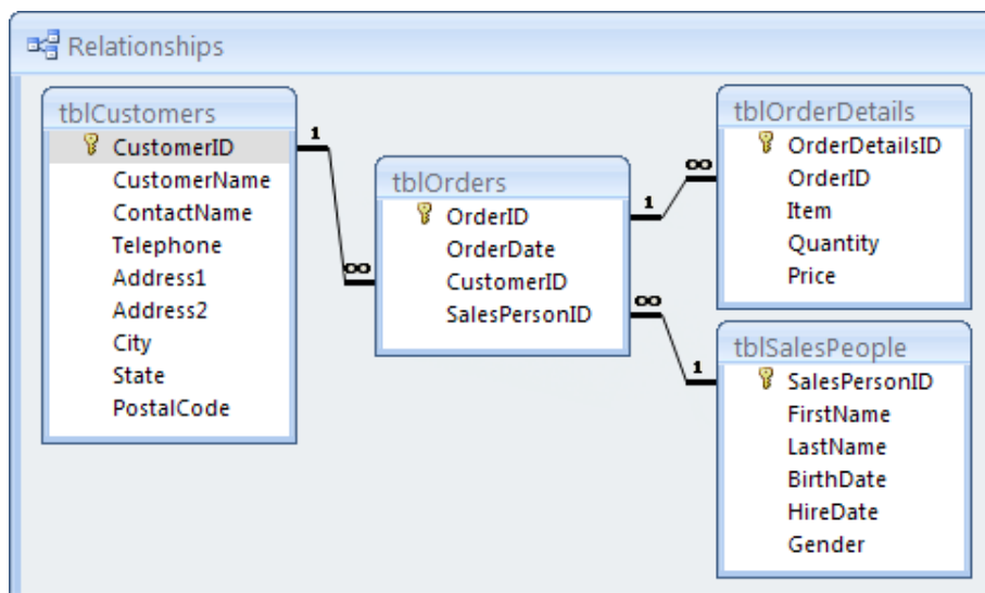
Fig. 1 The relationships window.
