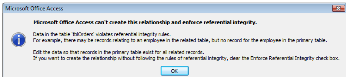
Fig. 10 Access can not enforce referential integrity when orphan records are already present.
