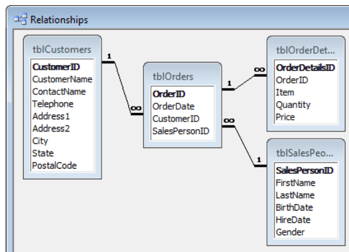
Fig. 1 The relationships window.
