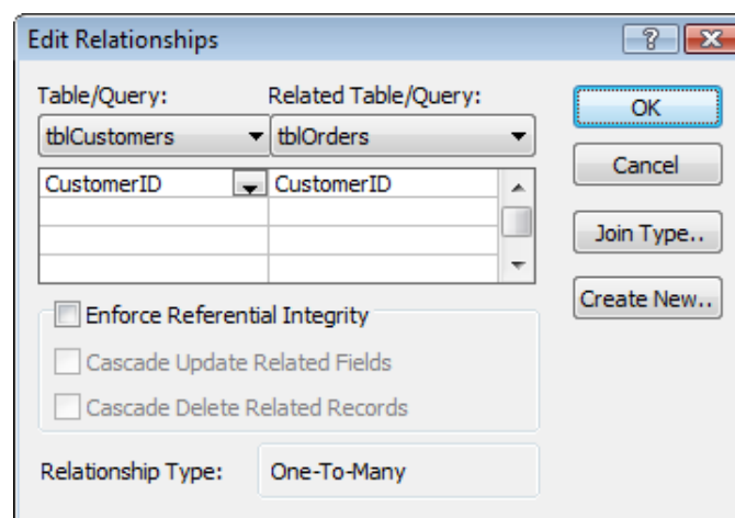
Fig. 7 The Edit Relationships dialog
